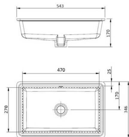
AGRES 53 X 34 UNDER COUNTER CERAMIC WASH BASIN
