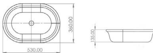
BLANCHE 53 X 36 TITANCAST ABOVE COUNTER BASIN
