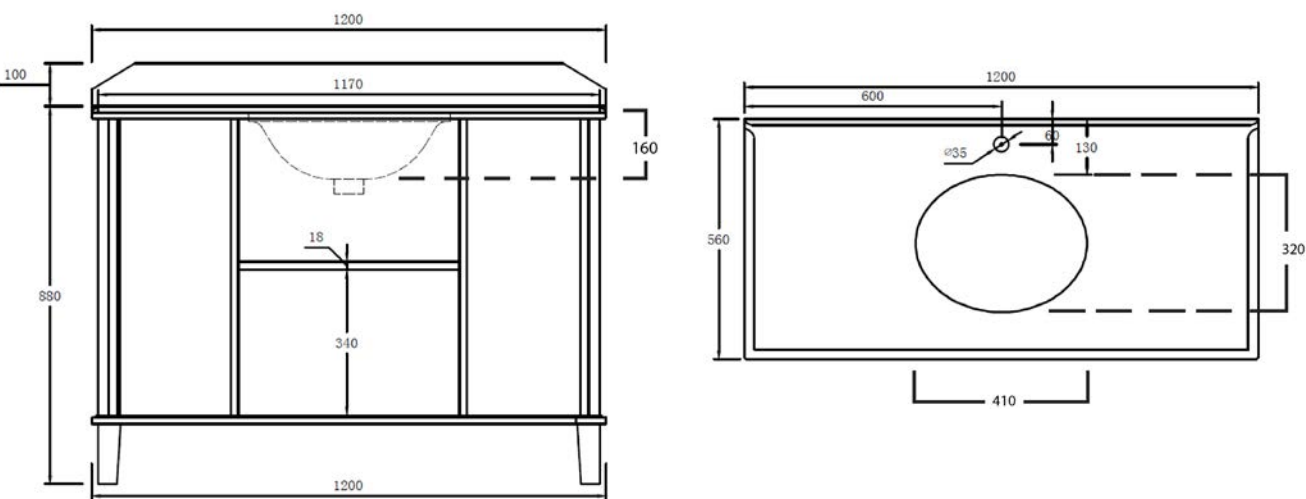
COVENTRY 120 X 55 SINGLE BOWL SATIN WHITE VANITY WITH REAL MARBLE TOP & CERAMIC UNDER COUNTER BASIN
