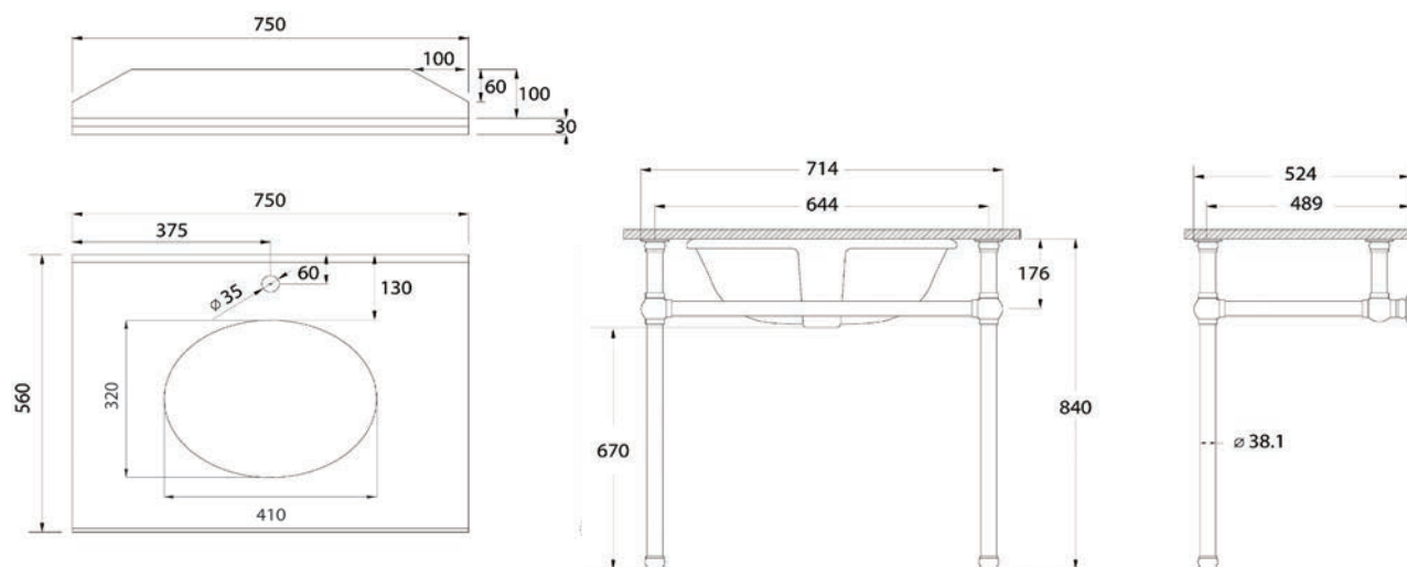
MAYER BASIN STAND WITH 75CM TOP
