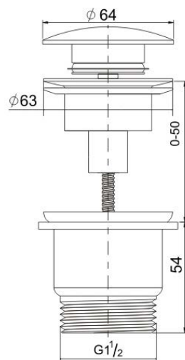
UNIVERSAL 32/40MM TWO PIECE MUSHROOM POP-UP WASTE
