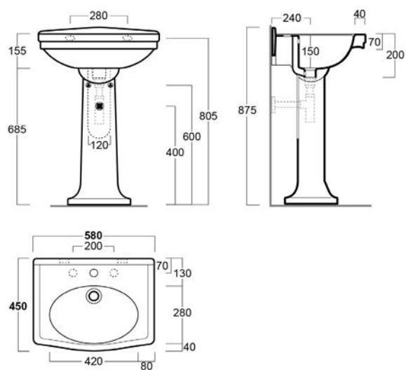
CLAREMONT 58 BASIN & PEDESTAL
