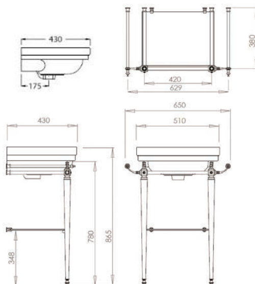
STAFFORD 51 X 43 BASIN STAND WITH GLASS SHELF
