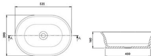
CAMBRIDGE 53 X 39 TITANCAST ABOVE COUNTER
