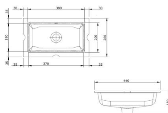
MINI AGRES 44 X 26 UNDER COUNTER CERAMIC WASH BASIN
