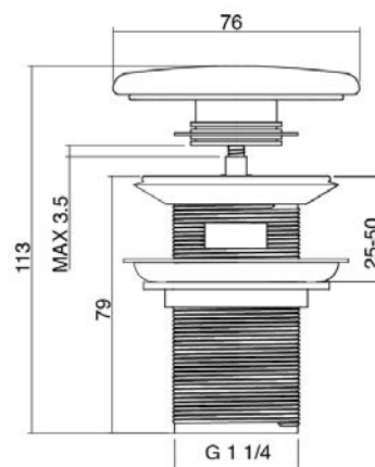
FIRECLAY BASIN WASTE
