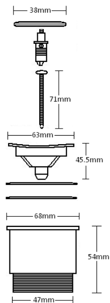
UNIVERSAL 32/40MM TWO PIECE BUTTON POP-UP WASTE -
