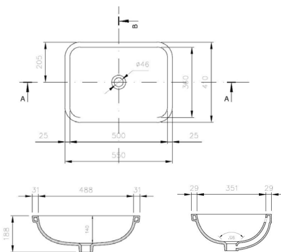
FINO 55 X 41 UNDERCOUNTER FINE FIRECLAY BASIN
