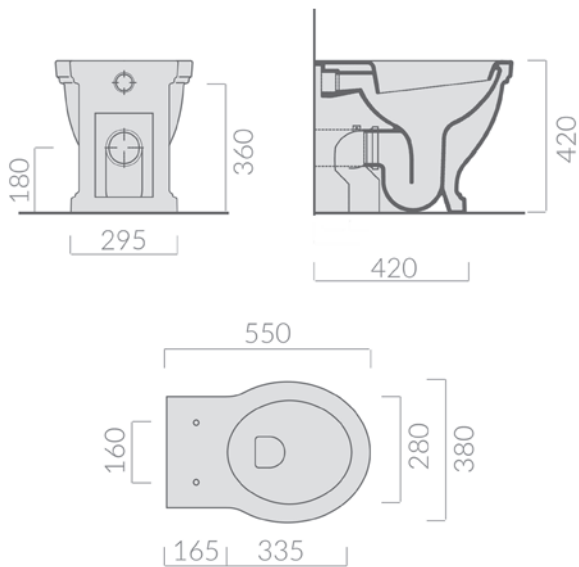
CLAREMONT FLOOR MOUNTED PAN
